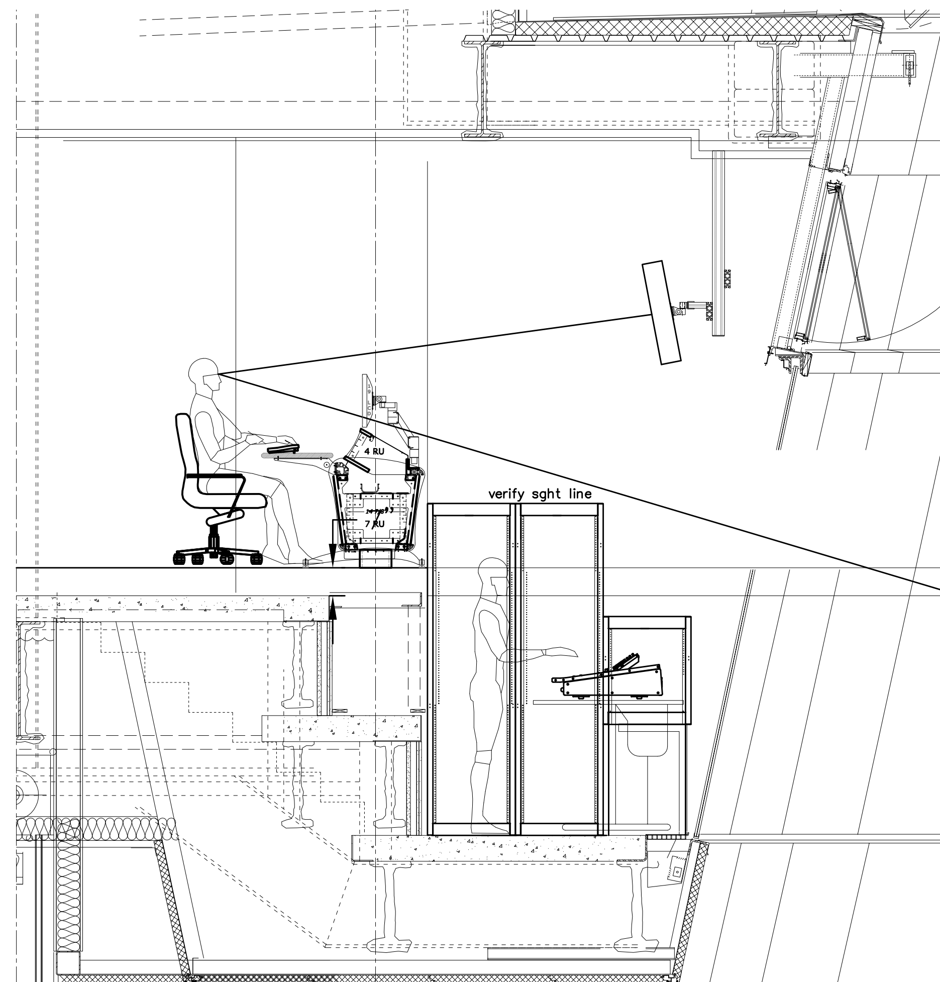
2 SECTION SCOREBOARD SCALE: 1/4" = 1'-0"
